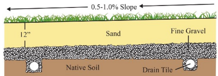
Conventional Sand-Based Athletic Field
